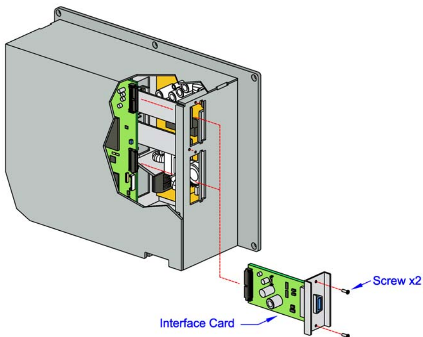
Figure 3-7, Interface Installation
